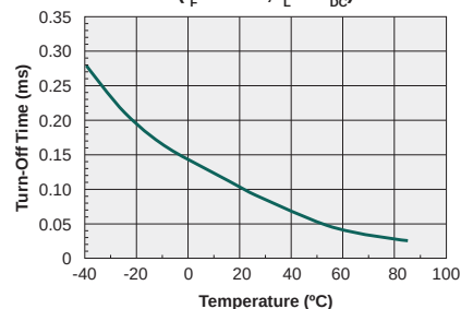
Typical Turn-Off Time vs. Temperature (I_F=10\text{mA}, I_L=1\text{A}_{\text{DC}})
