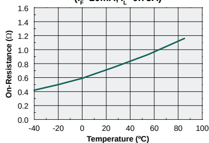
Typical On-Resistance vs. Temperature (I_F=20\text{mA}, I_L=0.75\text{A})
