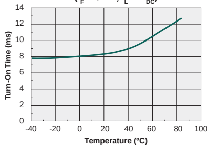
Typical Turn-On Time vs. Temperature (I_F=10\text{mA}, I_L=1\text{A}_{\text{DC}})
