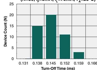
Typical Turn-Off Time (N=50, I_F=5\text{mA} , I_L=75\text{mA} , T_A=25^\circ\text{C} )
