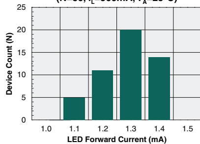
Typical I_F for Switch Operation (N=50, I_L=500\text{mA} , T_A=25^\circ\text{C} )
