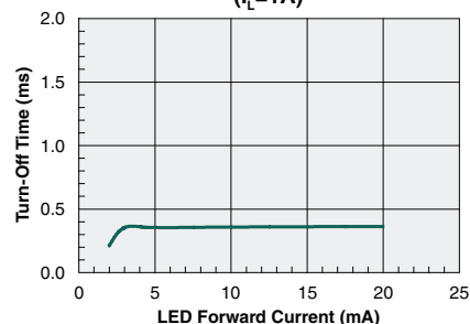
Typical Turn-Off Time vs. LED Forward Current ( I_L=1\text{A} )
