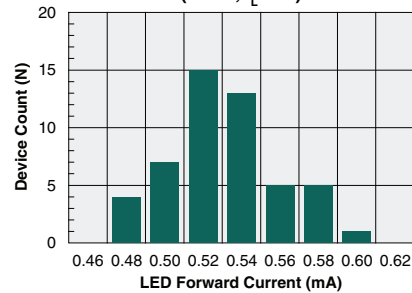
Typical I_F for Switch Operation (N=50, I_L=1A )
