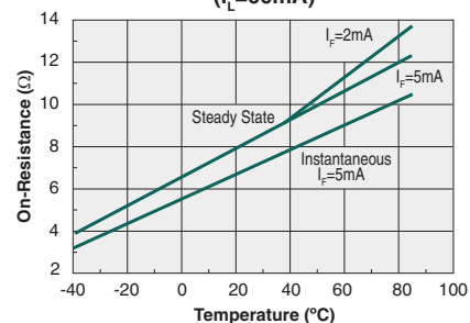
Typical On-Resistance vs. Temperature ( I_L = 60\text{mA} )
