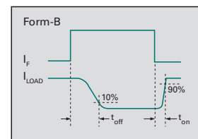
Switching Characteristics of Normally-Closed (Form-B) Devices
