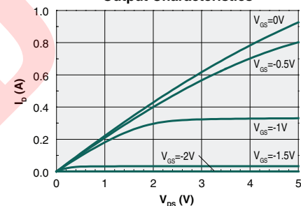
Output Characteristics
