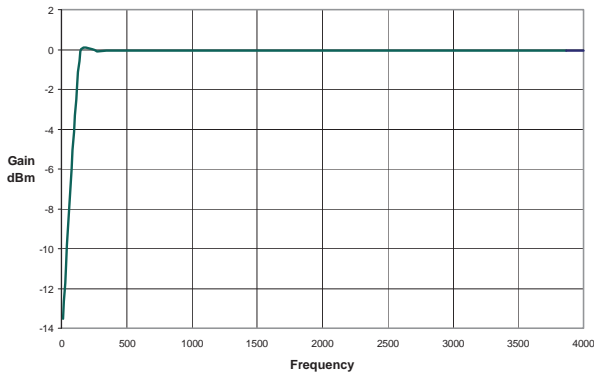
Figure 6. Receive Frequency Response at RX
