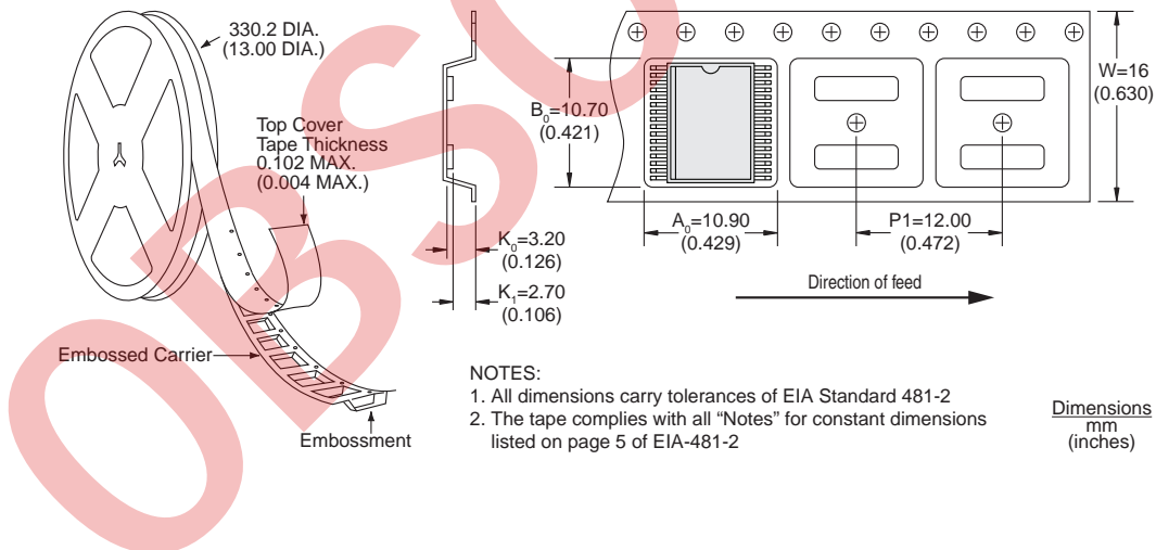
Figure 16. CPC5620ATR/CPC5621ATR Tape and Reel Dimensions
