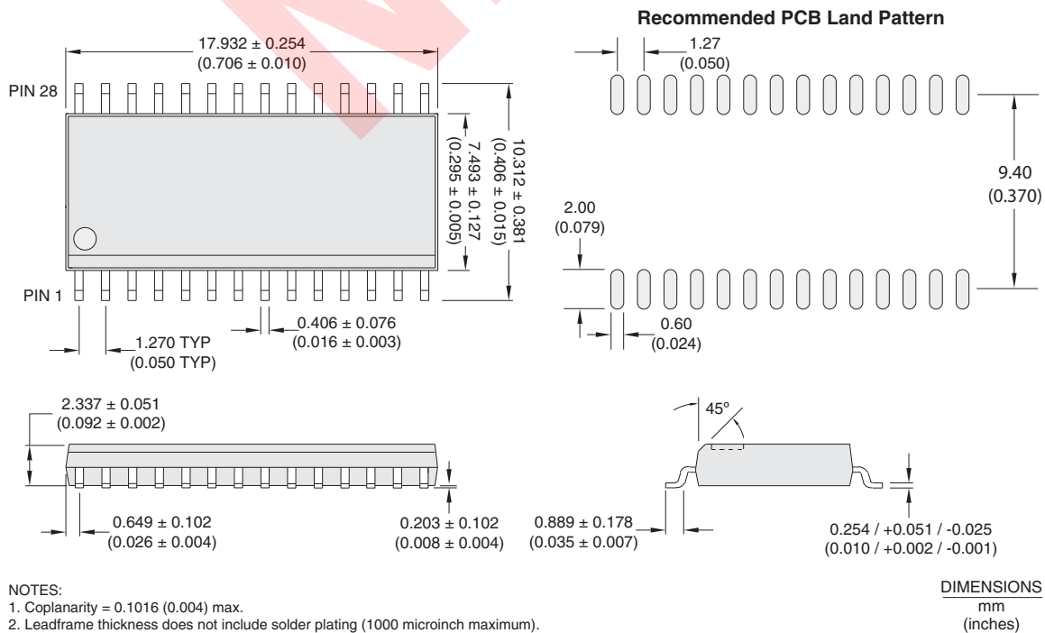
CPC7695Bx Package
