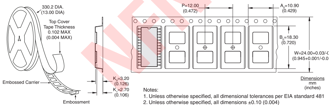
CPC7695BxTR Tape &amp; Reel
