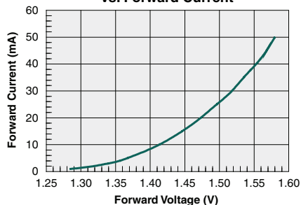
Typical LED Forward Voltage vs. Forward Current
