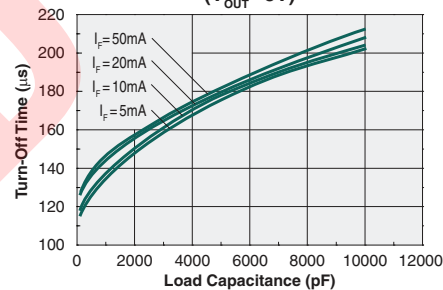
Turn-Off Time vs. Load Capacitance ( V_{OUT}=5\text{V} )
