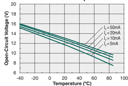
Open-Circuit Voltage vs. Ambient Temperature
