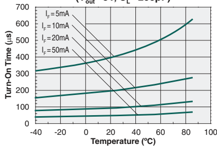
Turn-On Time vs. Ambient Temperature ( V_{OUT}=5\text{V} , C_L=200\text{pF} )
