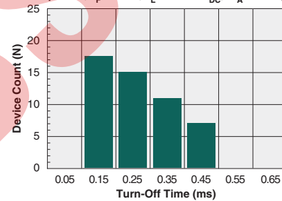
1-Form-A Typical Turn-Off Time (N=50, I_F=5\text{mA} , I_L=100\text{mA}_{DC} , T_A=25^\circ\text{C} )
