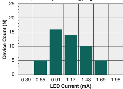
1-Form-A Typical I_F for Switch Operation (N=50, I_L=100\text{mA}_{DC} , T_A=25^\circ\text{C} )
