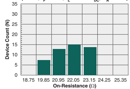
1-Form-A Typical On-Resistance Distribution (N=50, I_F=5\text{mA} , I_L=100\text{mA}_{DC} , T_A=25^\circ\text{C} )
