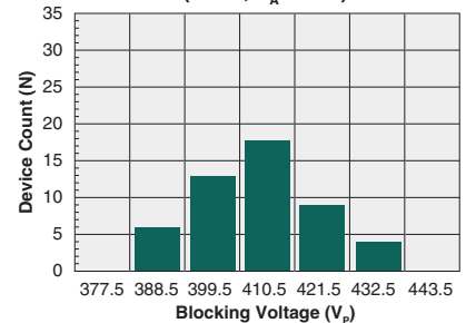
1-Form-A Typical Blocking Voltage Distribution (N=50, T_A=25^\circ\text{C} )
