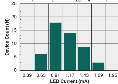
1-Form-A Typical I_F for Switch Dropout (N=50, I_L=100\text{mA}_{DC} , T_A=25^\circ\text{C} )
