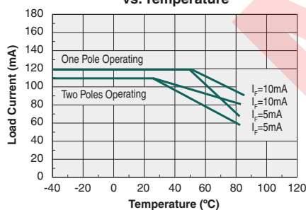
Maximum Continuous DC Load Current vs. Temperature
