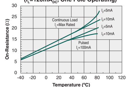
Typical On-Resistance vs. Temperature ( I_L = 120\text{mA}_{DC} , One Pole Operating)
