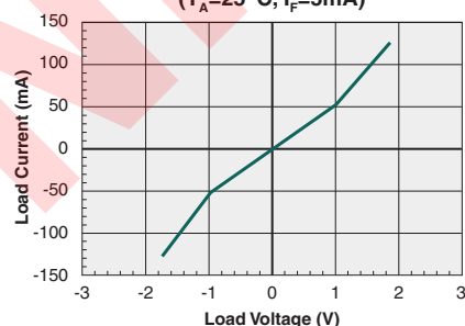
Typical Load Current vs. Load Voltage ( T_A = 25^{\circ}\text{C} , I_F = 5\text{mA} )
