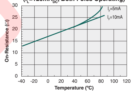
Typical On-Resistance vs. Temperature ( I_L = 120\text{mA}_{DC} , Both Poles Operating)
