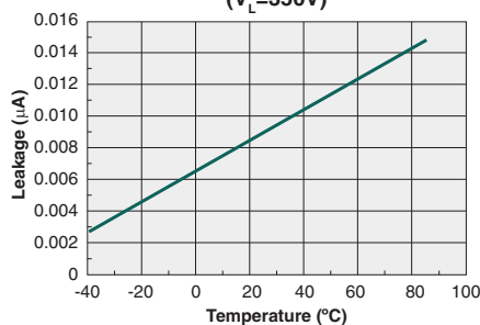
Typical Leakage vs. Temperature Measured across Pins 5&6, 7&8 ( V_L = 350\text{V} )
