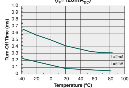
Typical Turn-Off Time vs. Temperature ( I_F=120\text{mA}_{DC} )
