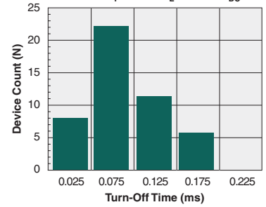
Typical Turn-Off Time (N=50, I F =5mA, I L =120mA DC )
