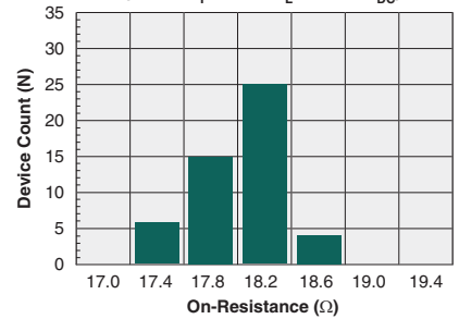
Typical On-Resistance Distribution (N=50, I F =2mA, I L =120mA DC )
