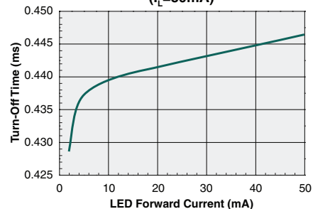
Turn-Off Time vs. LED Forward Current ( I_L=80\text{mA} )
