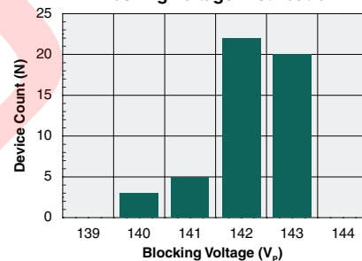
Blocking Voltage Distribution
