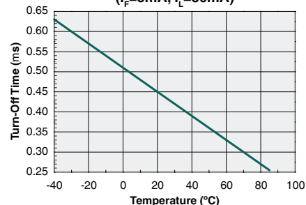
Turn-Off Time vs. Temperature ( I_F=5\text{mA} , I_L=80\text{mA} )
