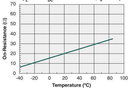
Typical On-Resistance vs. Temperature ( I_L = 50\text{mA}_{\text{DC}} Instantaneous, I_F = 5\text{mA} )
