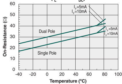
Typical On-Resistance vs. Temperature ( I_L = 120\text{mA}_{\text{DC}} )
