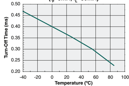
Typical Turn-Off Time vs. Temperature ( I_F=5\text{mA} , I_L=80\text{mA} )
