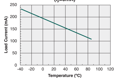
Form-B Maximum Load Current vs. Temperature ( I_F=0\text{mA} )
