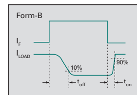
Switching Characteristics of Normally Closed Devices
