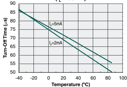
Form-A Typical Turn-Off Time vs. Temperature ( I_L=100\text{mA} )
