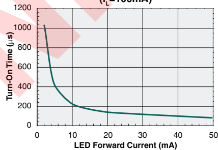
Form-A Typical Turn-On Time vs. LED Forward Current ( I_L=100\text{mA} )
