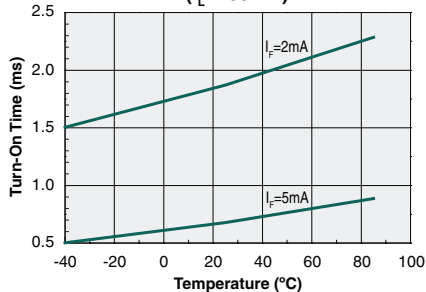
Form-A Typical Turn-On Time vs. Temperature ( I_L=100\text{mA} )
