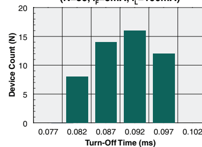
Form-A Typical Turn-Off Time (N=50, I_F=5\text{mA} , I_L=100\text{mA} )
