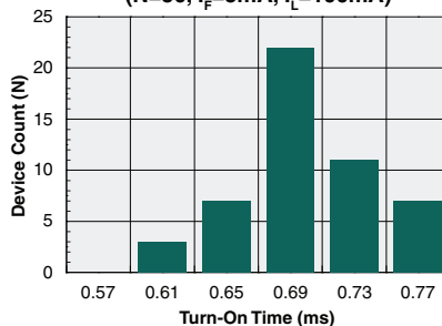
Form-A Typical Turn-On Time (N=50, I_F=5\text{mA} , I_L=100\text{mA} )
