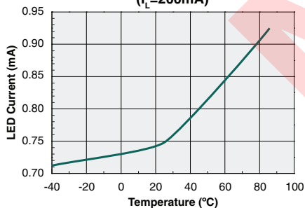
Form-A Typical I_F for Switch Operation vs. Temperature ( I_L=200\text{mA} )
