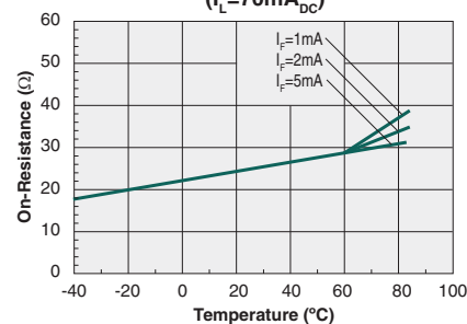
Typical On-Resistance vs. Temperature ( I_L = 70\text{mA}_{\text{DC}} )
