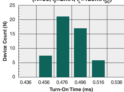
Typical Turn-On Time (N=50, I_F=2\text{mA} , I_L=120\text{mA}_{DC} )
