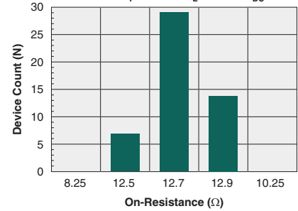
Typical On-Resistance Distribution (N=50, I_F=10\text{mA} , I_L=120\text{mA}_{DC} )
