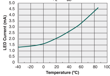
Typical I_F for Switch Dropout vs. Temperature ( I_L=1A_{DC} )
