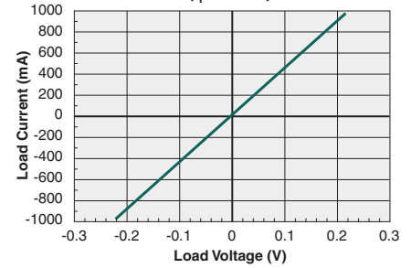
Typical Load Current vs. Load Voltage ( I_F=10mA )
