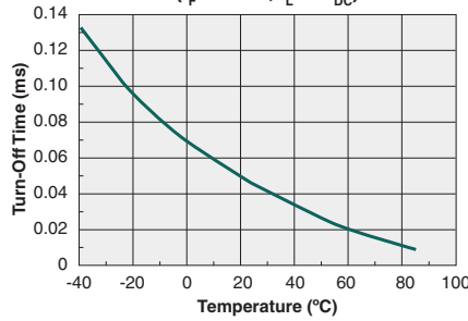
Typical Turn-Off Time vs. Temperature ( I_F=10mA, I_L=1A_{DC} )
