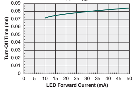
Typical Turn-Off Time vs. LED Forward Current ( I_L=1\text{A}_{DC} )
