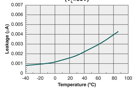
Typical Leakage vs. Temperature Measured across Pins 4&6 ( V_L=60V )
