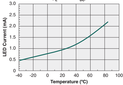
Typical I_F for Switch Operation vs. Temperature ( I_L = 170\text{mA}_{\text{DC}} )
