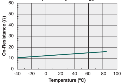
Typical On-Resistance vs. Temperature ( I_F=5\text{mA} , I_L=170\text{mA}_{DC} )
