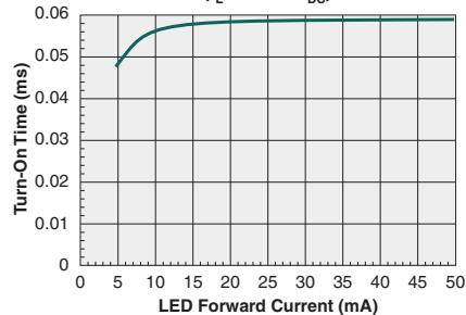
Typical Turn-On Time vs. LED Forward Current ( I_L=200\text{mA}_{DC} )
