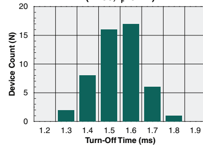
Typical Turn-Off Time (N=50, I_F=5\text{mA} )
