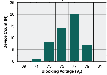
Typical Blocking Voltage Distribution (N=50, I_F=2mA )
