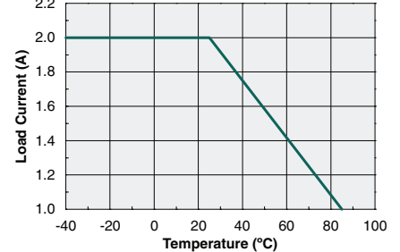
Maximum Load Current vs. Temperature DC-Only Configuration
