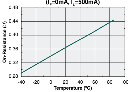
Typical On-Resistance vs. Temperature AC/DC Configuration
