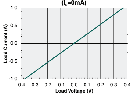
Typical Load Current vs. Load Voltage AC/DC Configuration
