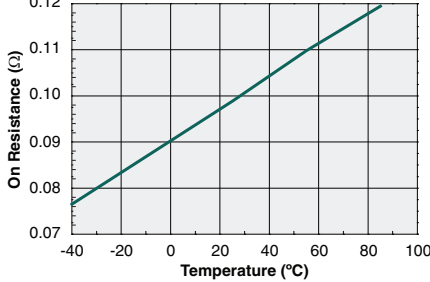
Typical On-Resistance vs. Temperature DC-Only Configuration
