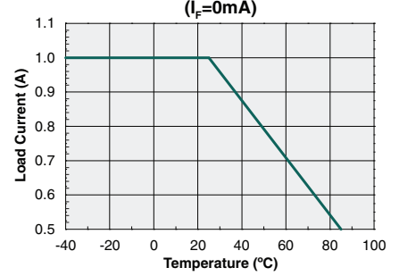
Maximum Load Current vs. Temperature AC/DC Configuration
