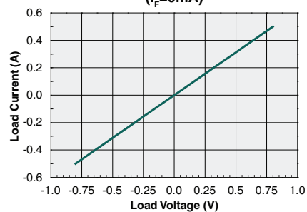
Typical Load Voltage vs. Load Current ( I_F=0\text{mA} )
