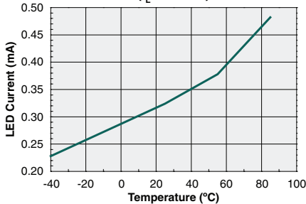
Typical LED Current to Operate vs. Temperature ( I_L=750mA )
