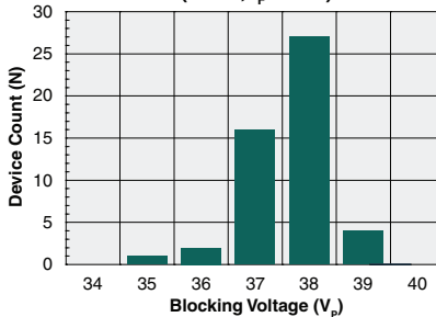
Typical Blocking Voltage Distribution (N=50, I_f=2mA )
