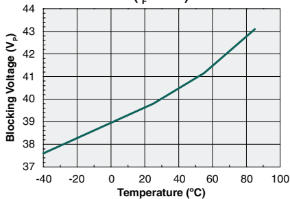
Typical Blocking Voltage vs. Temperature ( I_F=4mA )
