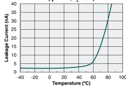
Leakage Current vs. Temperature Measured Across Pins 4 & 6 ( I_F=4mA , V_L=30V )
