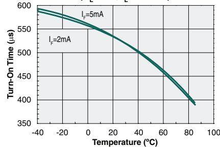
Typical Turn-On Time vs. Temperature ( V_L=10V , I_L=100mA )
