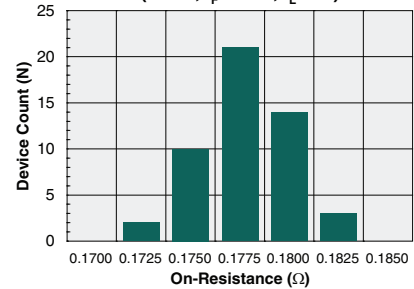
Typical On-Resistance Distribution (N=50, I_f=0mA , I_L=1A )
