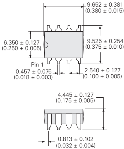
LCC120S
