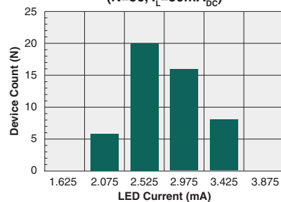
Typical I_F for Switch Operation (N=50, I_L=50\text{mA}_{DC} )
