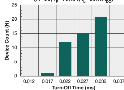
Typical Turn-Off Time (N=50, I_F=10\text{mA} , I_L=50\text{mA}_{DC} )
