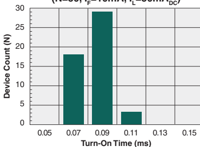
Typical Turn-On Time (N=50, I_F=10\text{mA} , I_L=50\text{mA}_{DC} )
