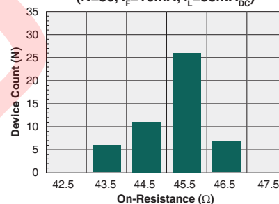
Typical On-Resistance Distribution (N=50, I_F=10\text{mA} , I_L=50\text{mA}_{DC} )
