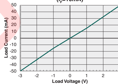
Typical Load Current vs. Load Voltage ( I_F=10\text{mA} )
