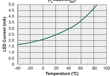
Typical I_F for Switch Operation vs. Temperature ( I_L=50\text{mA}_{\text{DC}} )
