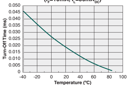
Typical Turn-Off Time vs. Temperature ( I_F=10\text{mA} , I_L=50\text{mA}_{\text{DC}} )
