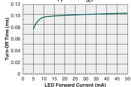
Typical Turn-Off Time vs. LED Forward Current ( I_F=150\text{mA}_{DC} )
