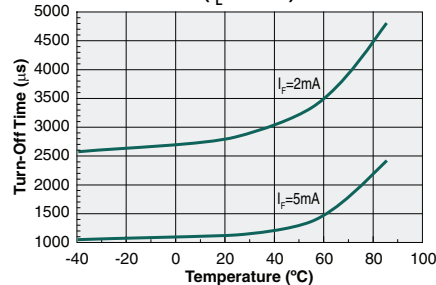
Turn-Off Time vs. Temperature ( I_L=75mA )
