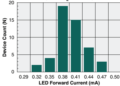
Typical LED Forward Current to Activate (N=50, I_L=100mA )
