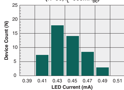
Typical I_F for Switch Operation (N=50, I_L=600\text{mA}_{DC} )
