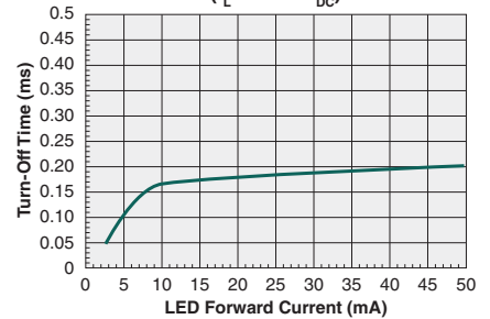
Typical Turn-Off Time vs. LED Forward Current ( I_L=200\text{mA}_{DC} )
