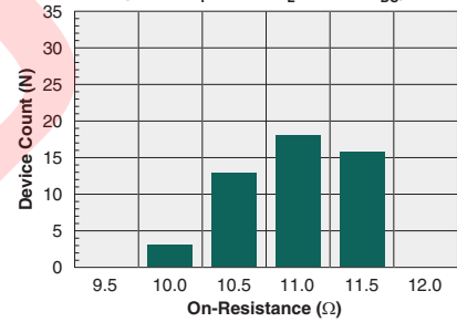
Typical On-Resistance Distribution (N=50, I_F=5\text{mA} , I_L=200\text{mA}_{DC} )
