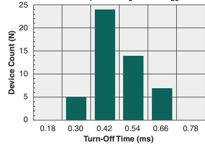
Typical Turn-Off Time (N=50, I_F=5\text{mA} , I_L=200\text{mA}_{DC} )
