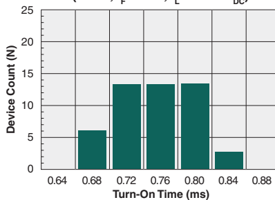
Typical Turn-On Time (N=50, I_F=2\text{mA} , I_L=100\text{mA}_{DC} )
