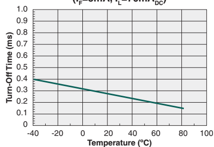
Typical Turn-Off Time vs. Temperature ( I_F = 5\text{mA} , I_L = 70\text{mA}_{\text{DC}} )
