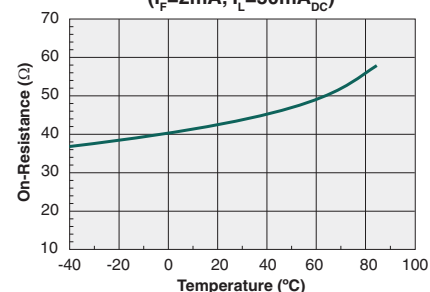
Typical On-Resistance vs. Temperature ( I_F = 2\text{mA} , I_L = 50\text{mA}_{\text{DC}} )
