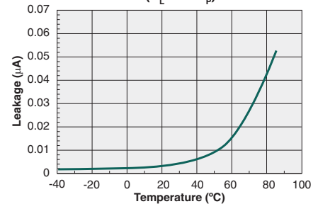
Typical Leakage vs. Temperature Measured across Pins 4&6 ( V_L=300V_P )
