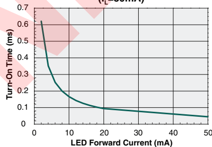
Typical Turn-On Time vs. LED Forward Current ( I_L=30\text{mA} )
