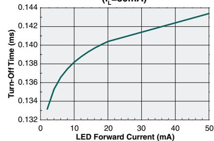
Typical Turn-Off Time vs. LED Forward Current ( I_L=30\text{mA} )
