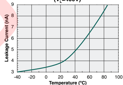
Leakage Current vs. Temperature Measured Across Pins 5&6 ( V_L=400\text{V} )
