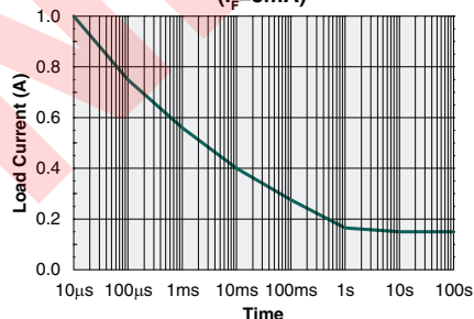
Energy Rating Curve, Single Pole ( I_F=5\text{mA} )
