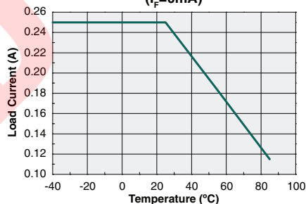
Maximum Load Current vs. Temperature - DC Configuration ( I_F=0\text{mA} )
