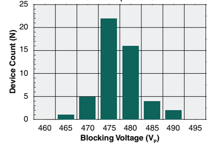
Typical Blocking Voltage Distribution (N=50, I_F=2mA )
