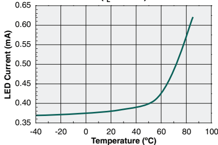
LED Current to Operate vs. Temperature ( I_L=75mA )
