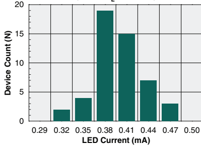
Typical LED Current to Operate (N=50, I_L=100mA )
