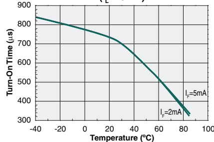
Typical Turn-On Time vs. Temperature ( I_L=75mA )
