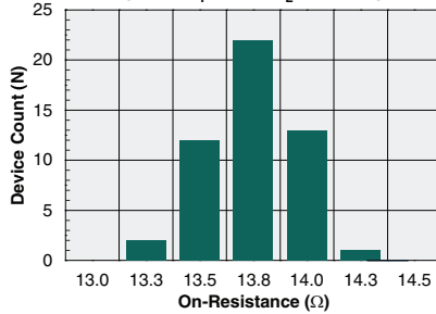
Typical On-Resistance Distribution (N=50, I_F=0mA , I_L=100mA )
