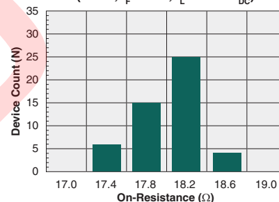
Typical On-Resistance Distribution (N=50, I_F=2\text{mA} , I_L=120\text{mA}_{DC} )
