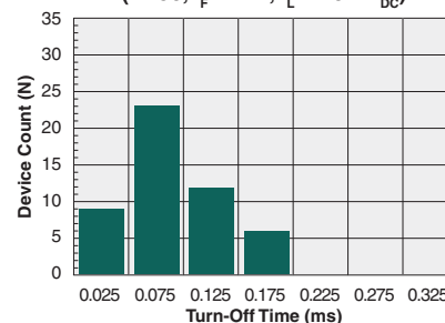
Typical Turn-Off Time (N=50, I_F=2\text{mA} , I_L=120\text{mA}_{DC} )
