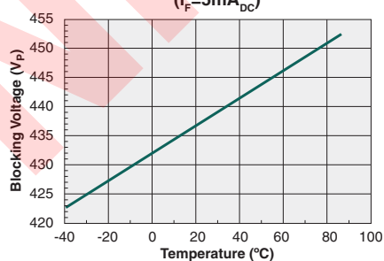
Typical Blocking Voltage vs. Temperature ( I_F = 5\text{mA}_{\text{DC}} )
