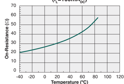
Typical On-Resistance vs. Temperature ( I_L = 100\text{mA}_{\text{DC}} )
