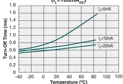
Typical Turn-Off Time vs. Temperature ( I_L = 100\text{mA}_{\text{DC}} )
