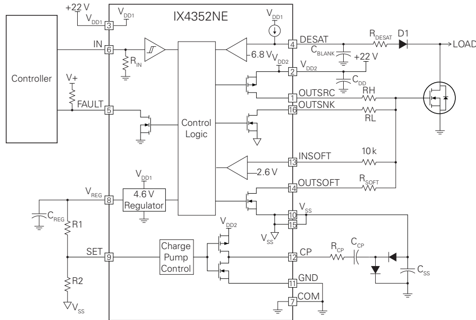
Figure 1 IX4352NE Typical Application Circuit
