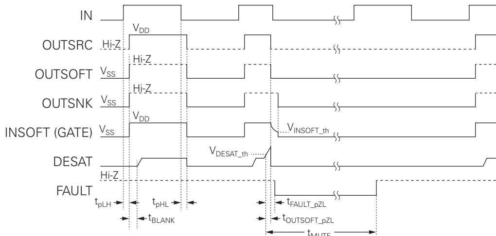
Figure 2 IX4352NE Logic Diagram
