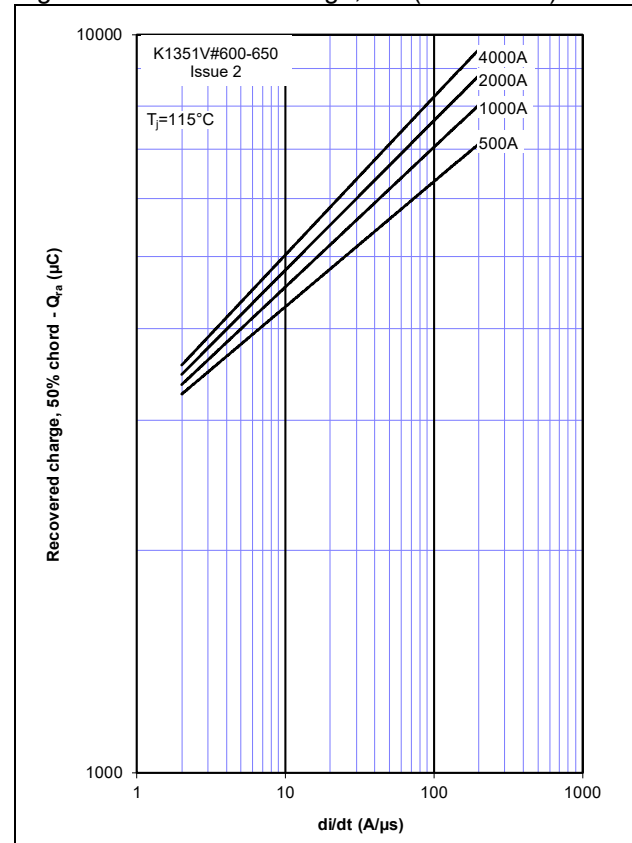
Figure 6 - Recovered charge, Q_{ra} (50% chord) ( \mu\text{C} )
