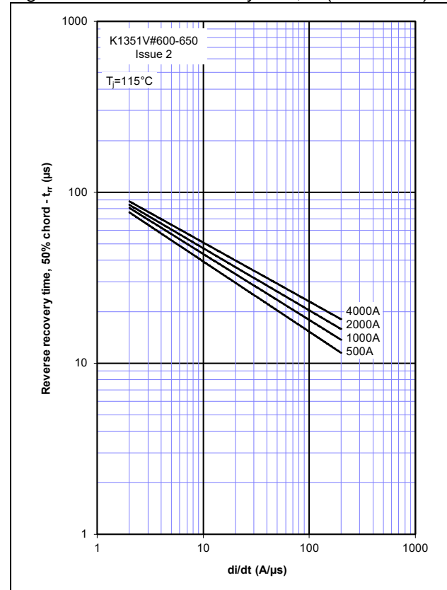
Figure 8 - Maximum recovery time, t_{rr} (50% chord) ( \mu\text{s} )
