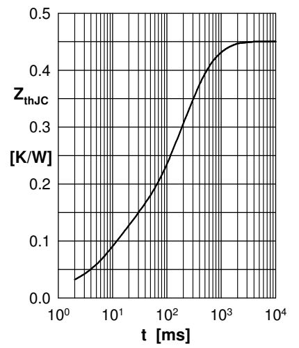
Fig. 8 Transient thermal impedance junction to case
