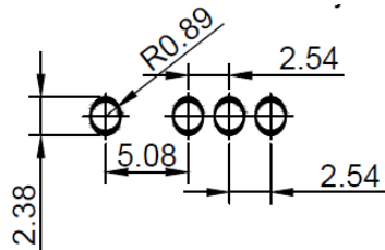
Recommended Hole Pattern Layout:
