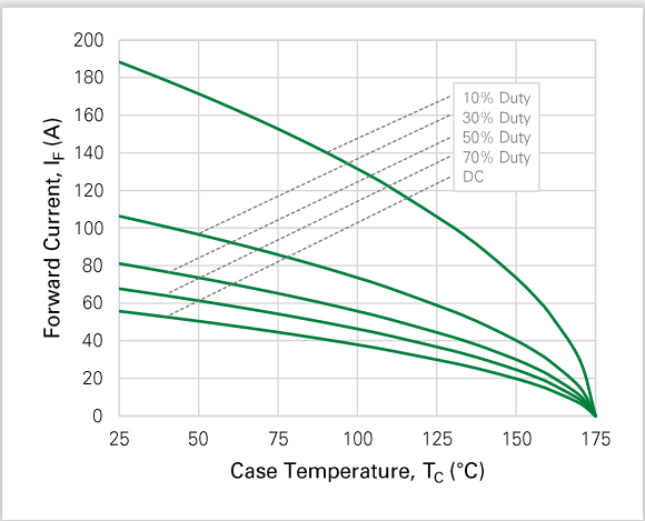
Figure 4. Current Derating
