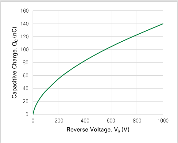
Figure 6. Capacitive Charge vs. Reverse Voltage
