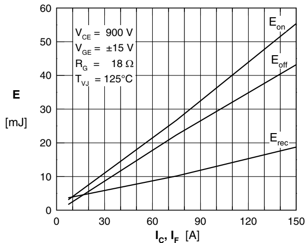
Fig. 13 Typ. turn on energy & switching times versus collector current
