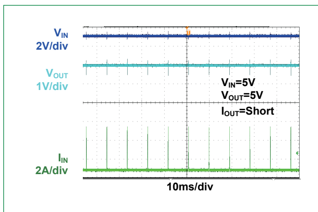
Figure 11 - Short Protection ( 5V_{IN} , R_{limit} = \text{float} )
