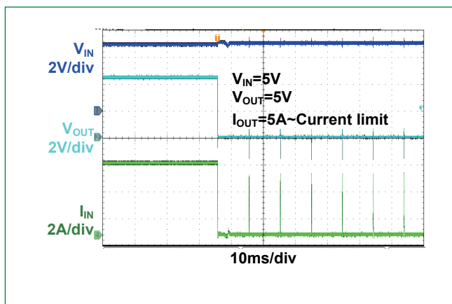
Figure 9 - Current Limit ( 5V_{IN} , R_{limit} = \text{float} )
