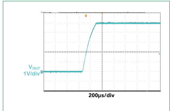
Figure 8 - Soft Start ( 5V_{IN} , I_O = 0 A)
