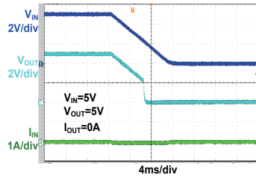
Figure 4 - Vin Off (5V IN , I O = 0 A)
