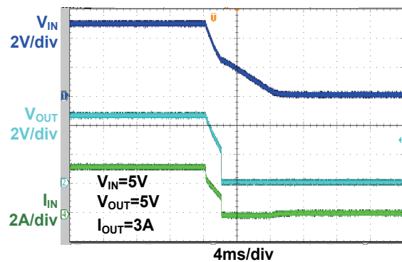
Figure 6 - V IN Off (5V IN , I O = 3 A)
