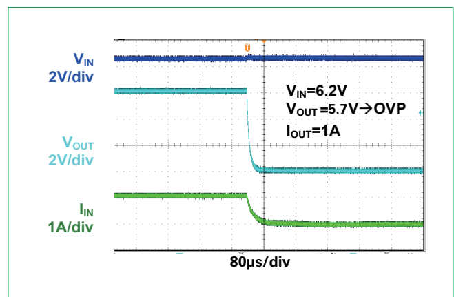
Figure 12 - Over Voltage Protection ( 5V_{IN} Application, I_O = 1 A)
