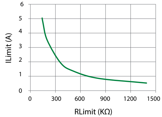
Figure 2 - RLimit vs. Ilimit (5V IN Application)
